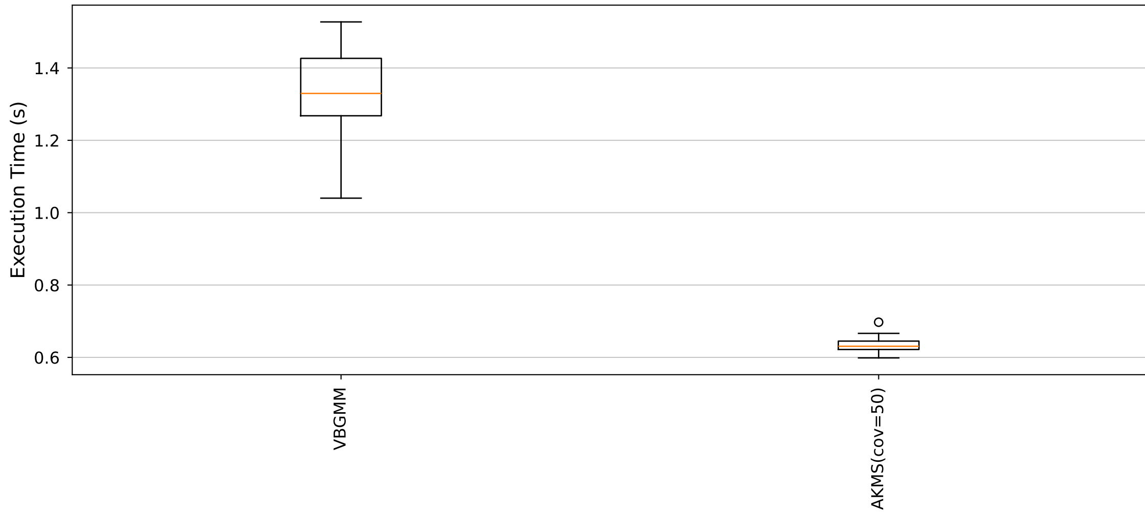
YARA Rules Execution Time Distribution (Cluster33_Size6 dataset)
